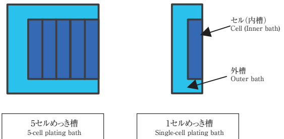
図3 めっき槽構造 Fig. 3 Configuration of plating bath
