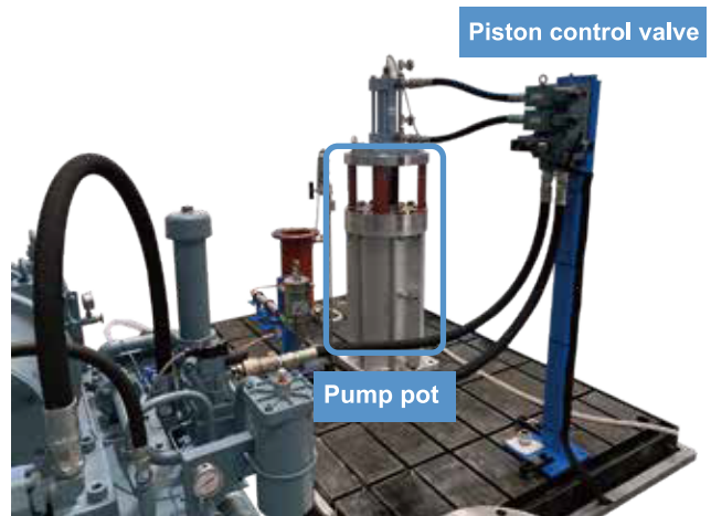
Hydraulic system unit
