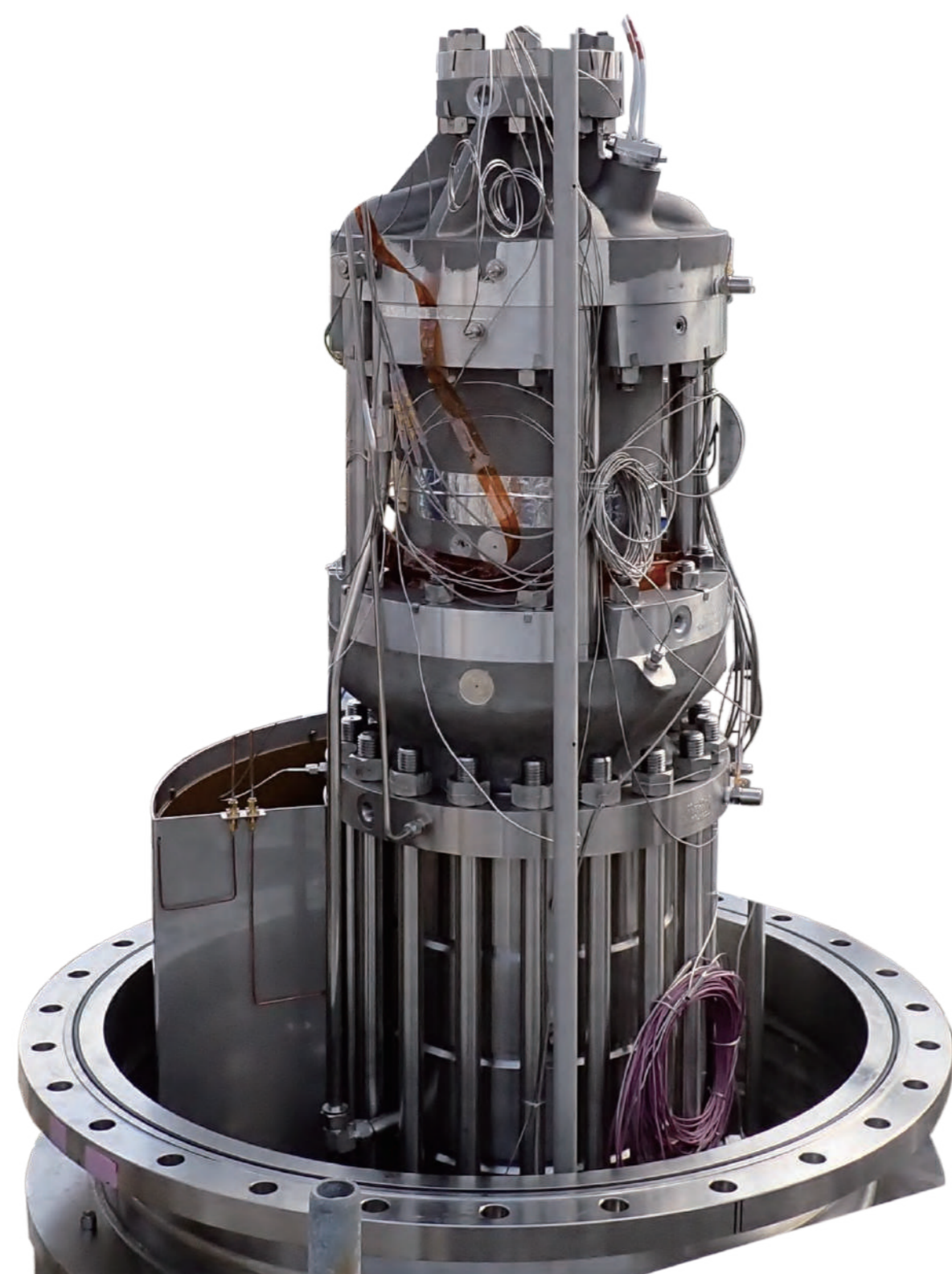
Prototype of Liquid Hydrogen Pump
