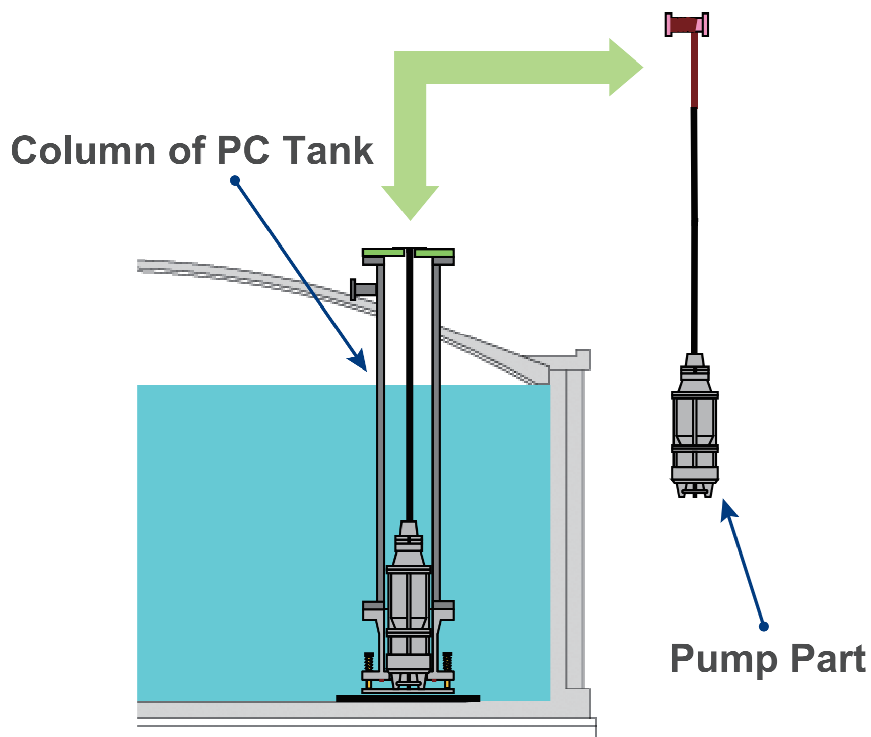
Image of Pump Detachment and Attachment to PC Tank
