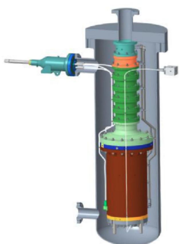
Liquid CO 2 Expander
