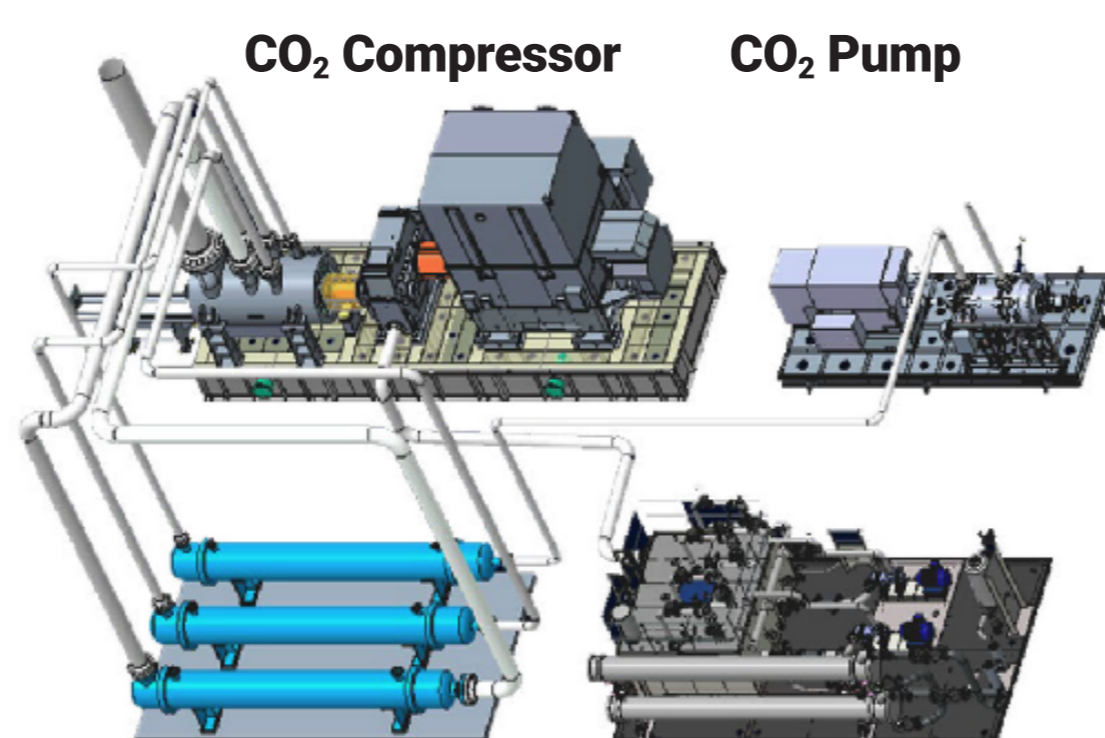
CO 2 Phase Hybrid Compressor Pump Solution
