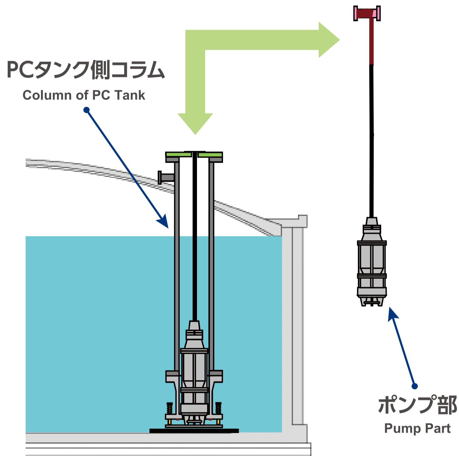
PCタンクへのポンプ脱着イメージ Image of pump detachment and attachment to PC Tank
