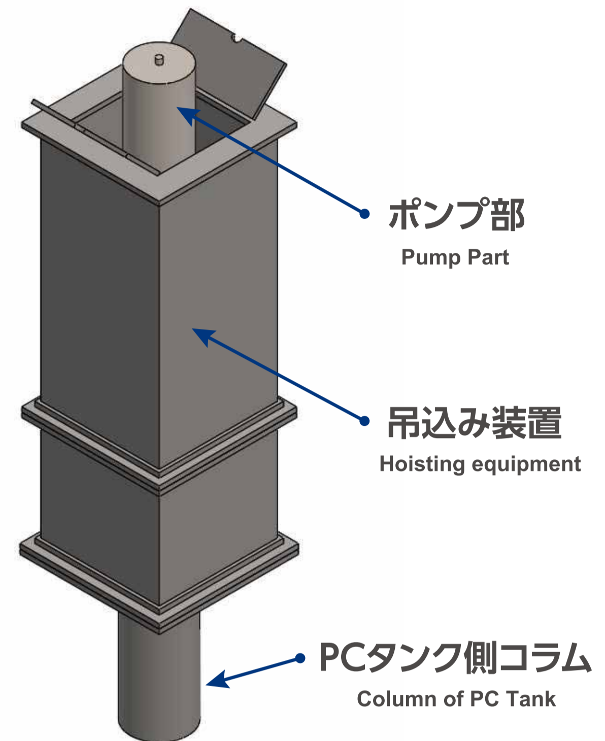
吊込み装置イメージ(開発中) Image of hoisting equipment (under development)
