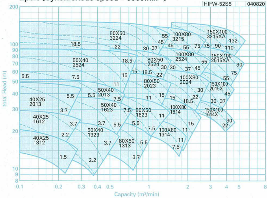
2pole [Synchronous speed : 3000min -1 ]
