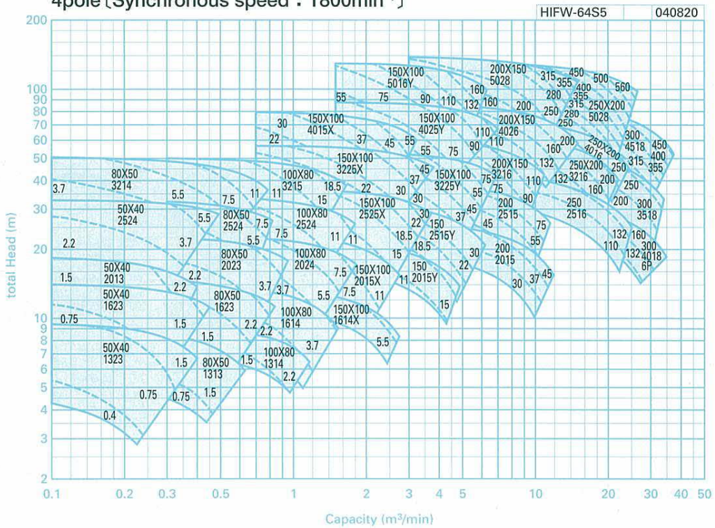
4pole [Synchronous speed : 1800min -1 ]
